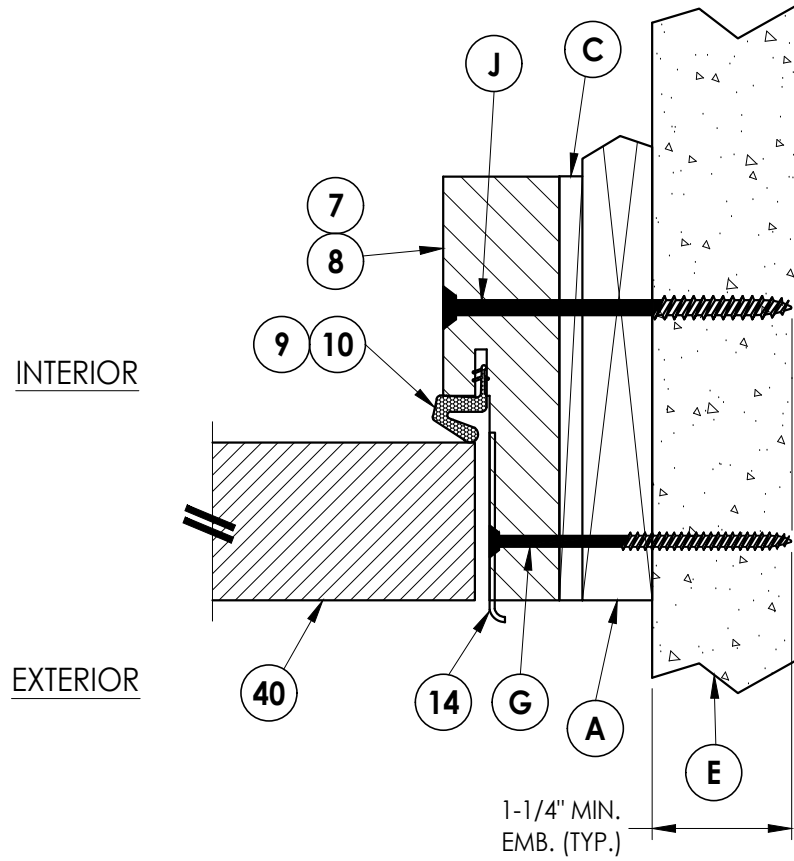
3 3 HORIZONTAL CROSS SECTION Shown w/ 1X sub-buck
