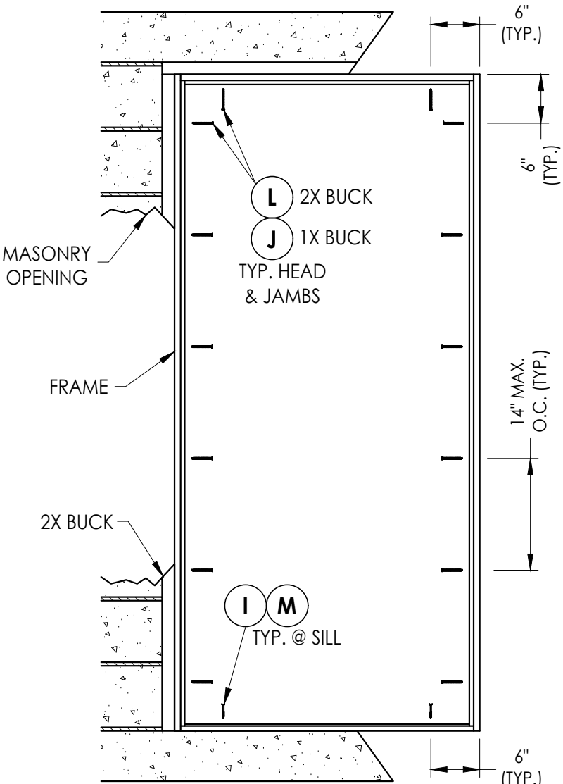
FRAME ANCHORING
